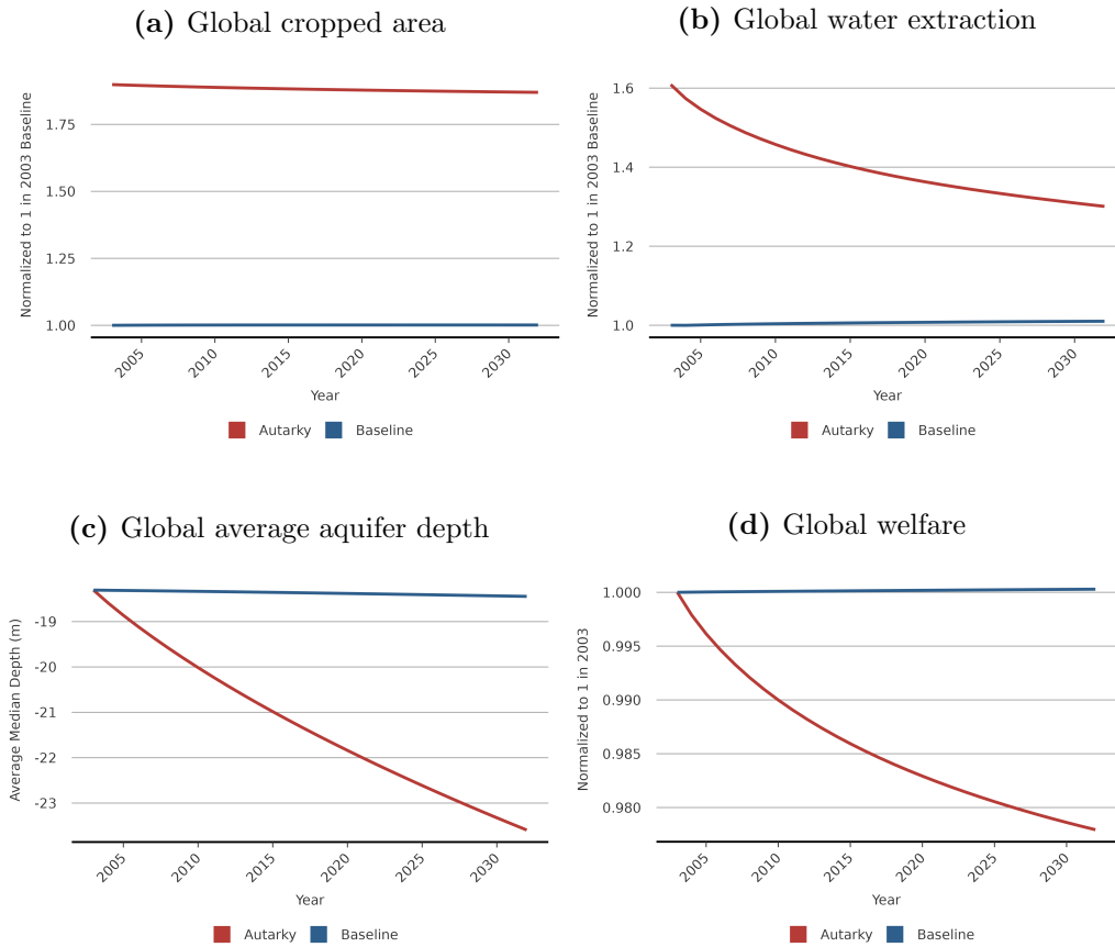
Figure 8: Simulated Impact of Agricultural Trade on Global Agriculture, Water, and Welfare Over Time
