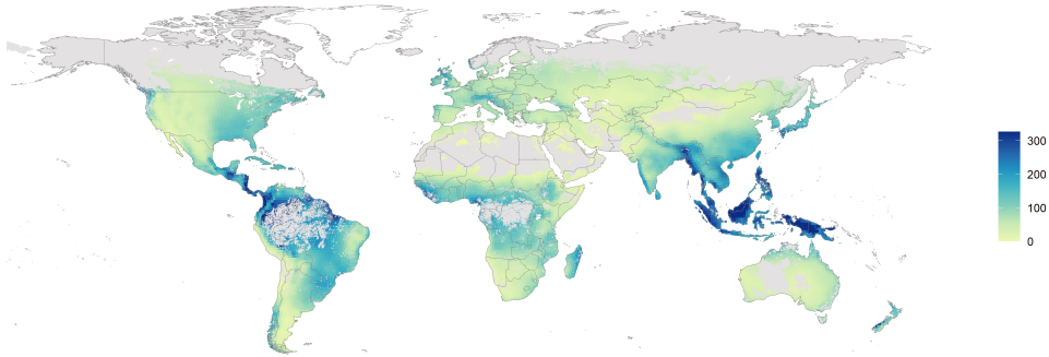
(b) Average Groundwater Table Depth (meters below land surface)
