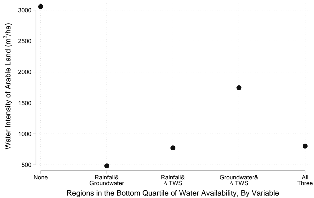
Figure 4: Water Intensity of Arable Land Use in Water-Stressed Regions
