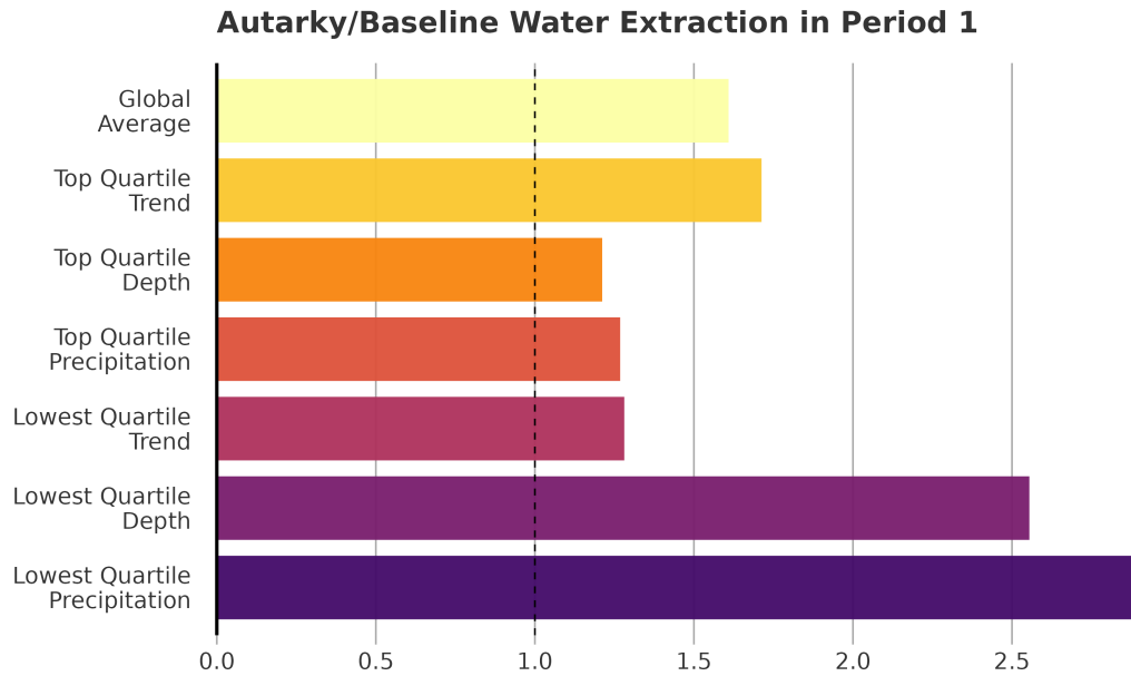
(b) Heterogeneity by Initial Water Resource Characteristics
