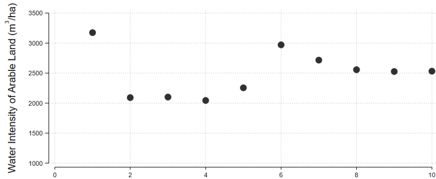
(c) Deciles of Trends in Total Water Storage ( \rightarrow Gaining More Water)
