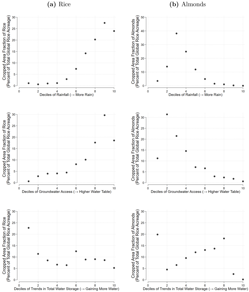
Figure 2: Cropped Area Fraction by Decile of Water Variables
