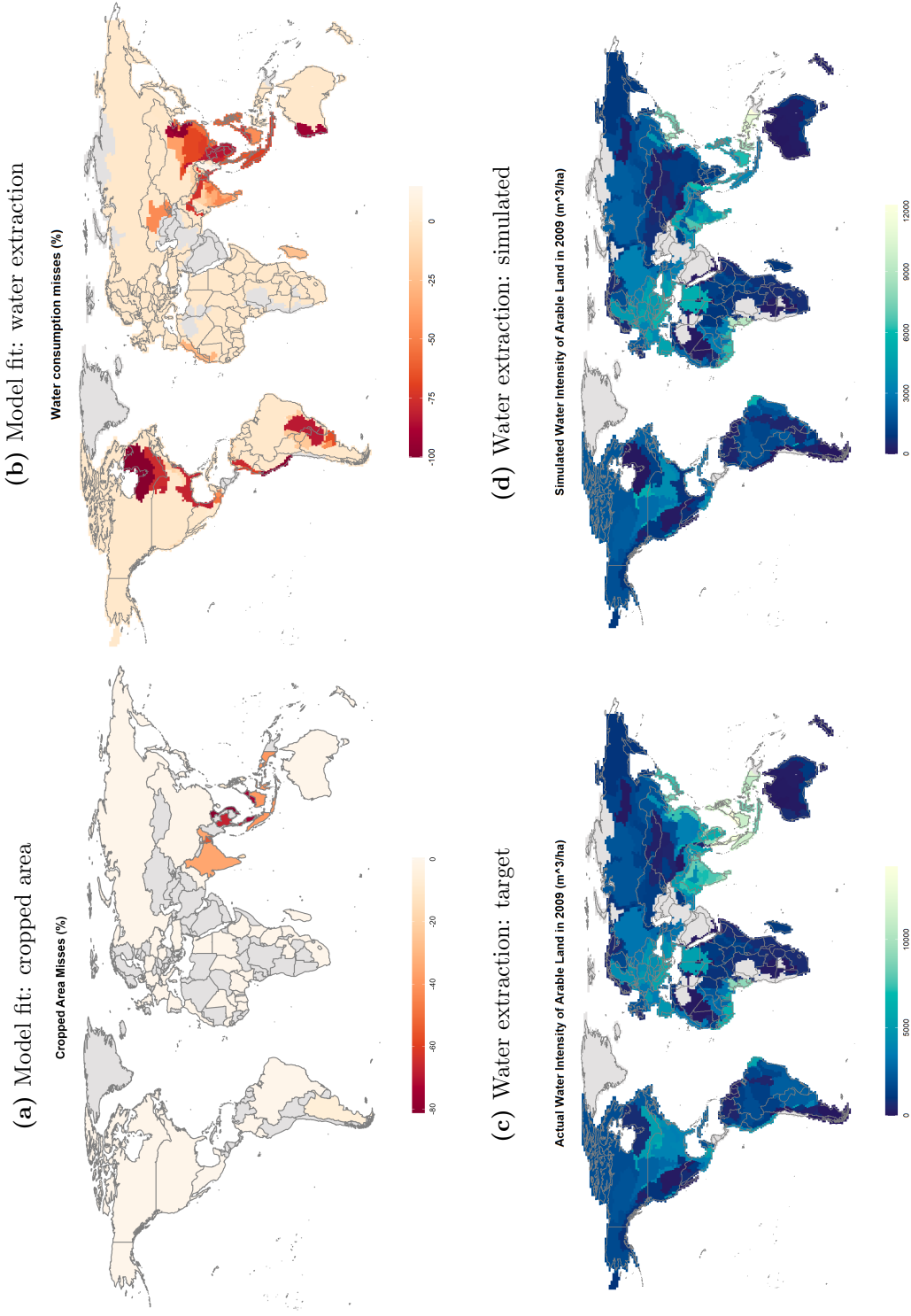
Figure 6: Simulated Model Fit for Cropped Area and Water Extraction
