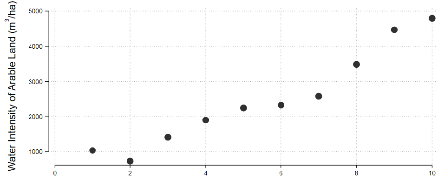
(b) Deciles of Groundwater Access ( \rightarrow Higher Water Table)
