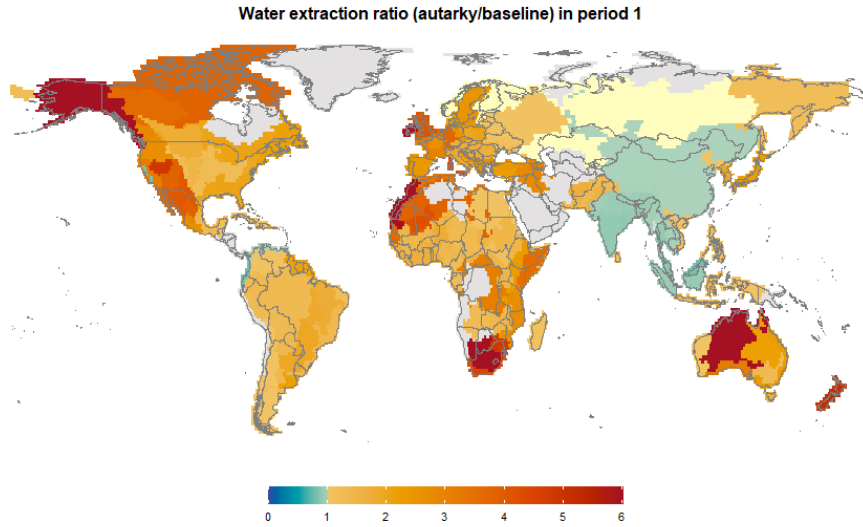
(b) Heterogeneity by Initial Water Resource Characteristics
