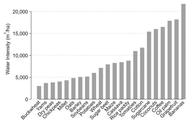
(c) Water intensity of 22 crops included in the model
