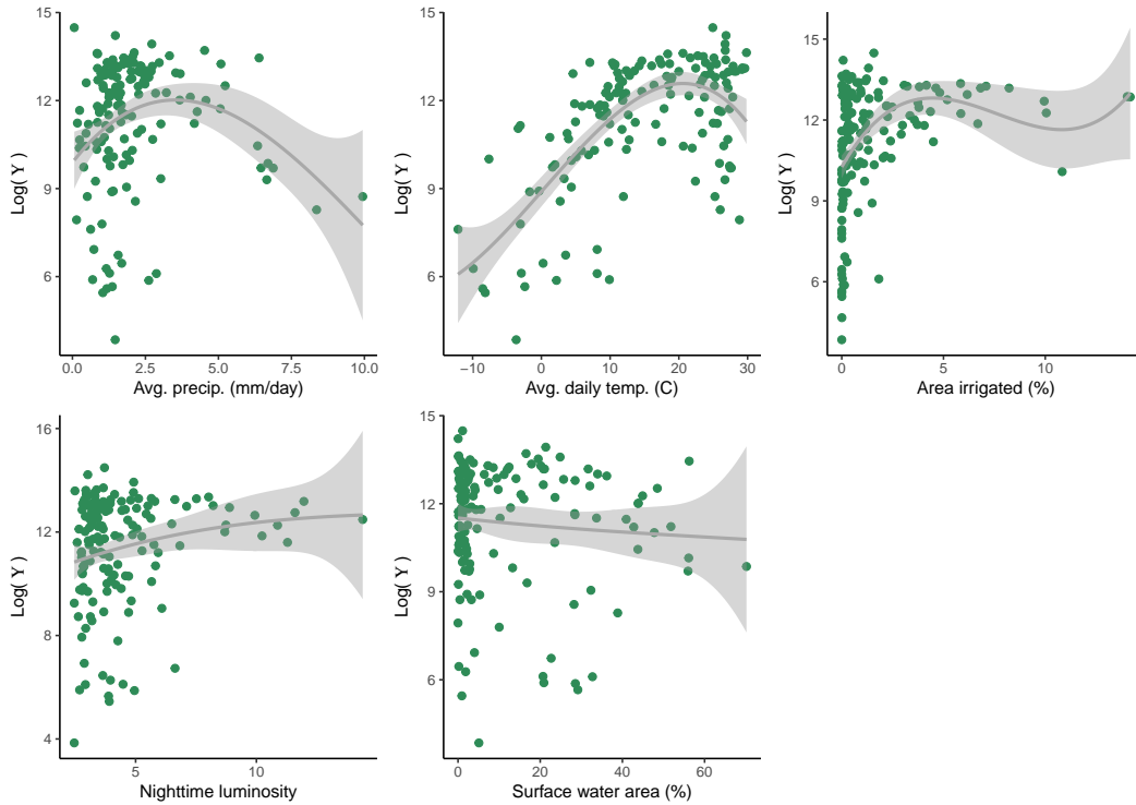
Figure 7: Correlations Between Model Parameters Mapping Aquifer Depth to Extraction Productivity ( \Upsilon ) and Climate and Economic Covariates
