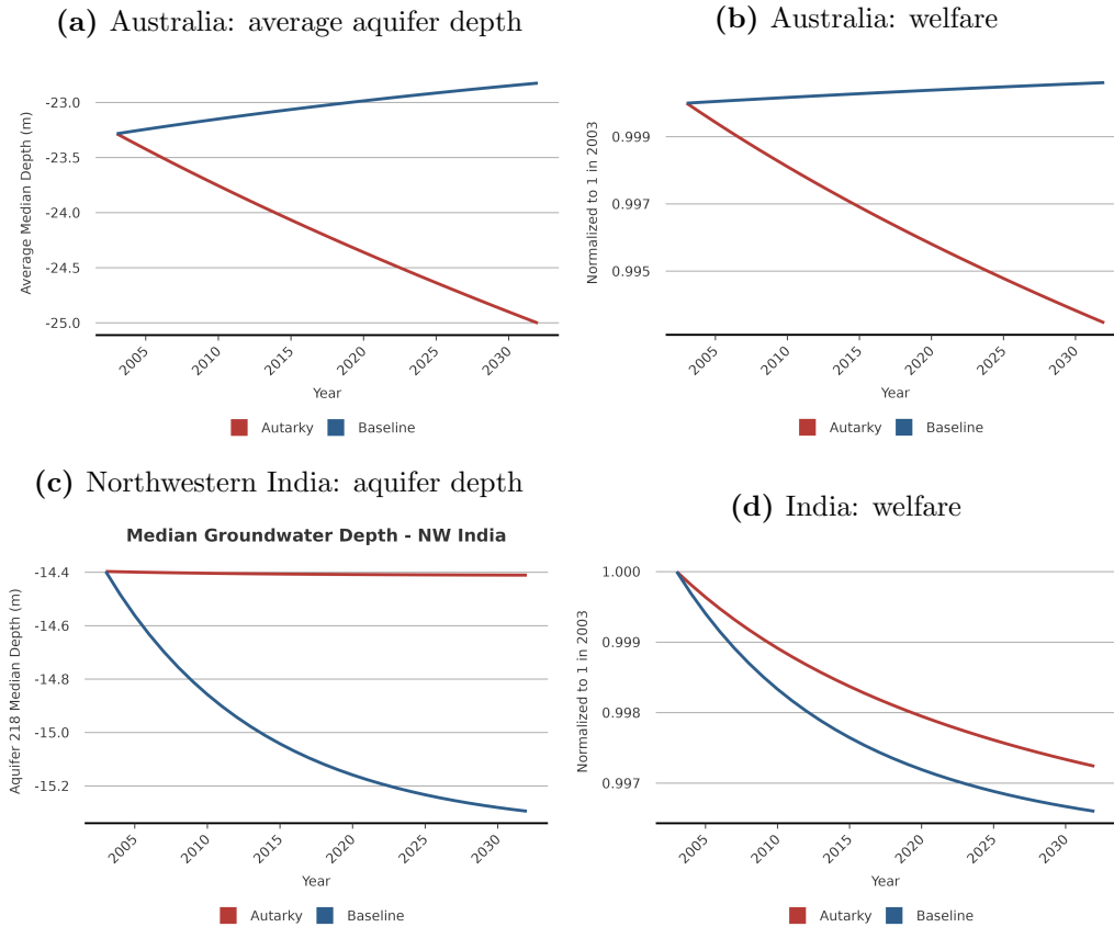
Figure 11: Simulated Impact of Agricultural Trade on Water and Welfare in Select Regions Over Time
