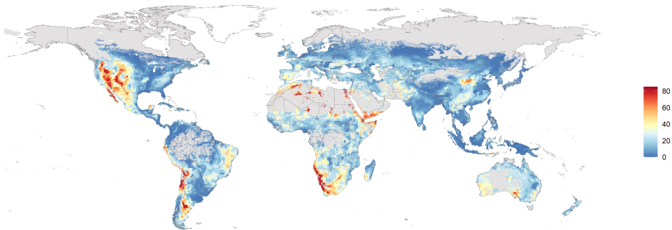
(c) Change in Total Water Storage (cm/year)
